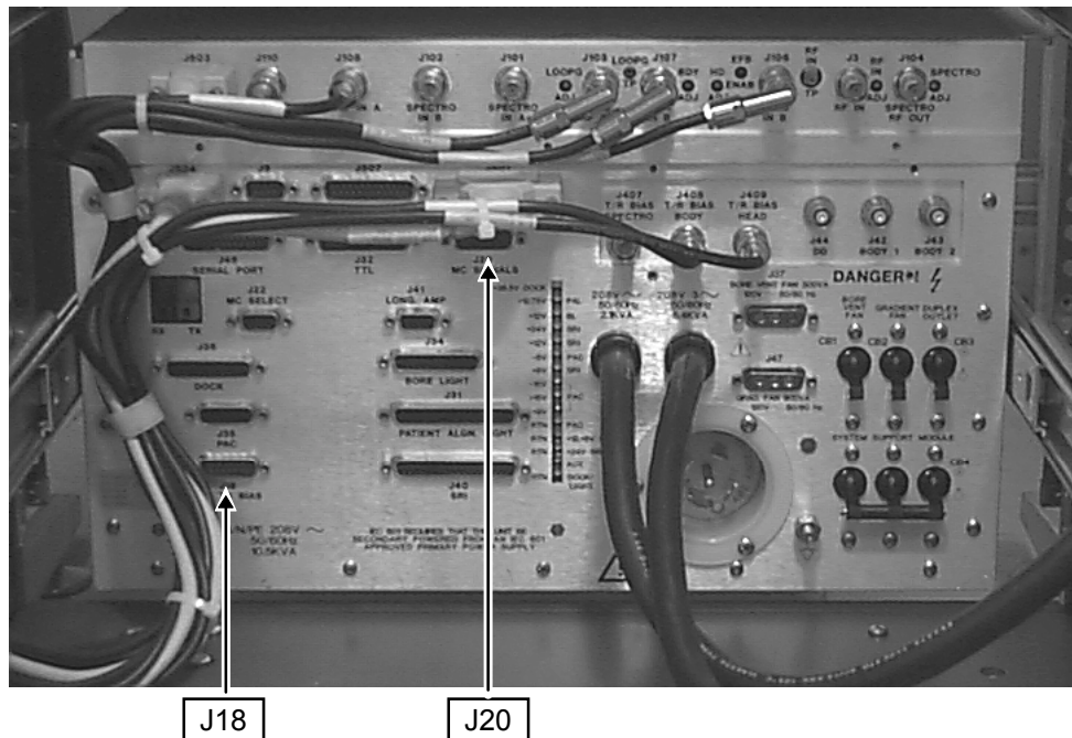
CABLES CONNECTED TO CORRECT LOCATIONS — MULTI-COIL ILLUSTRATION 6-2
