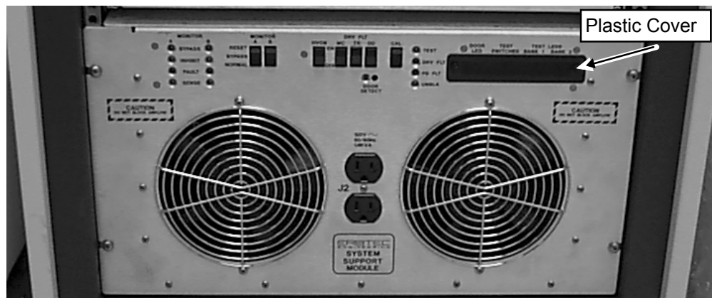
TEST SWITCH AND TEST LEDs WINDOW ILLUSTRATION 6-1
