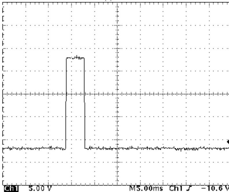
HEAD TR SCOPE WAVEFORM SEEN AT TP22 (HTR-OUT) ILLUSTRATION 5-6
