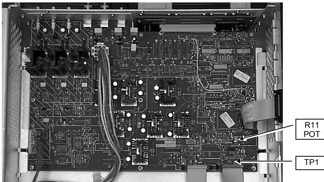
MULTI-COIL ADJUSTMENT/ –5VDC AT TP1 ILLUSTRATION 6-3
