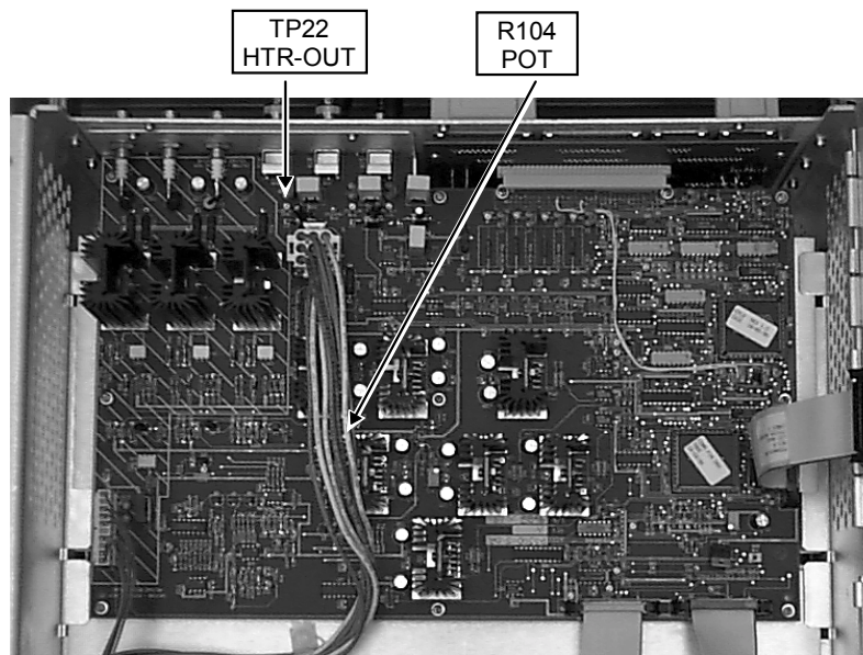
TR VOLTAGE ADJUSTMENT/HEAD TR TEST POINT ILLUSTRATION 5-5
