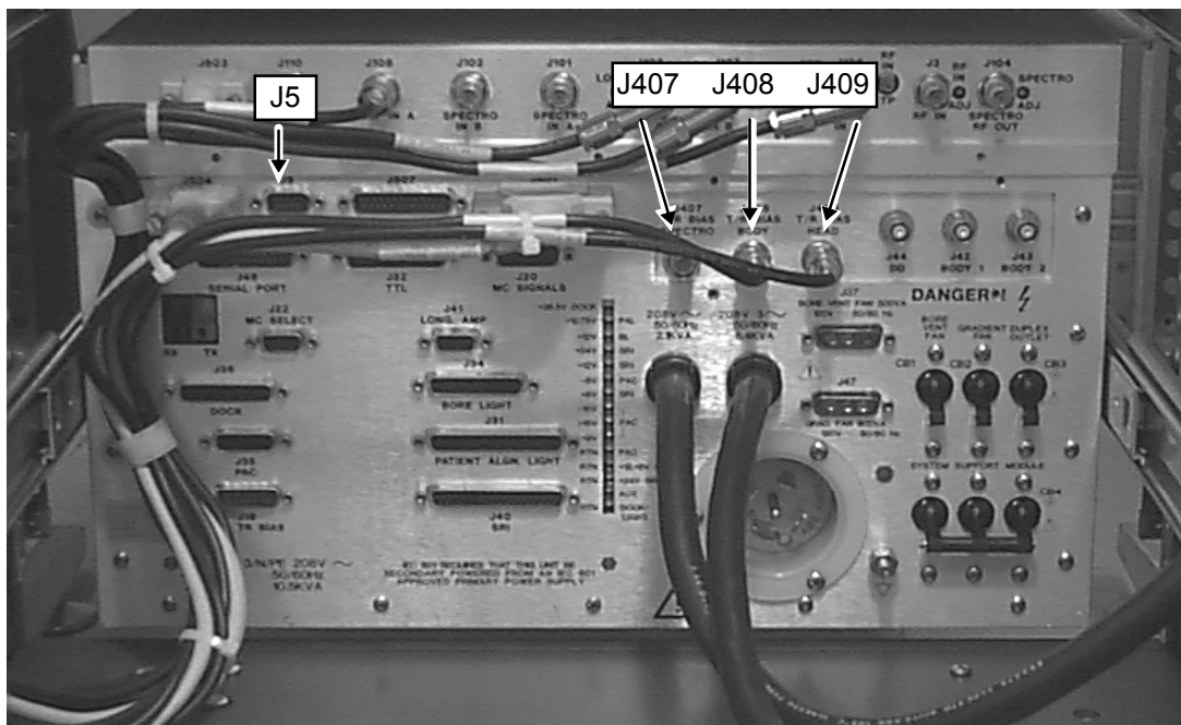
CABLES LOCATIONS ON SSM ILLUSTRATION 5-1
