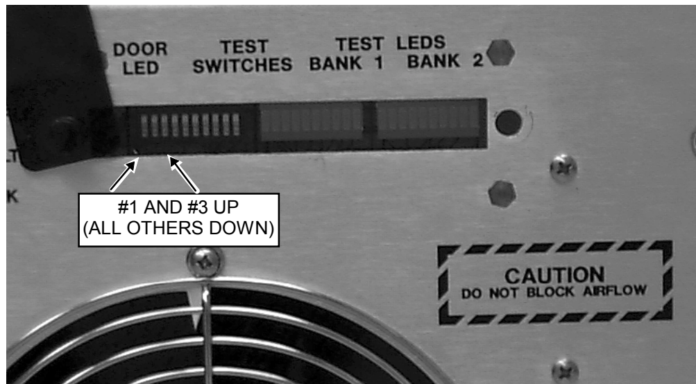
DIP SWITCH CONFIGURATION ILLUSTRATION 5-2
