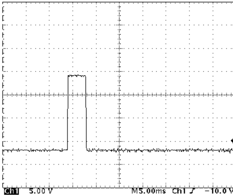
BODY TR SCOPE WAVEFORM SEEN AT TP18 (BTR-OUT) ILLUSTRATION 5-4
