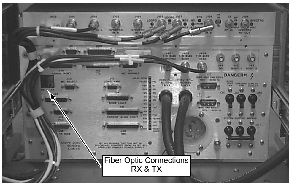
FIBER OPTIC CABLE CONNECTIONS ILLUSTRATION 7-1
