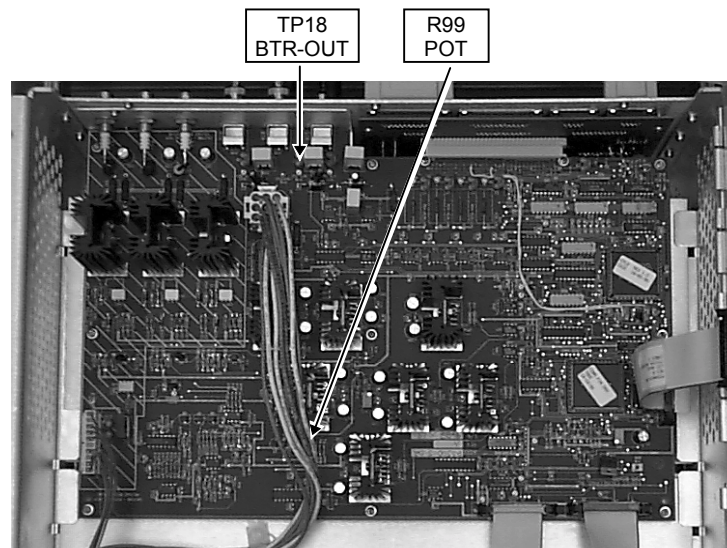
TR VOLTAGE ADJUSTMENT/BODY TR TEST POINT ILLUSTRATION 5-3
